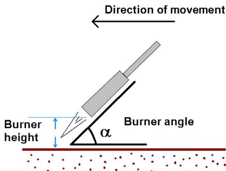
Figure 5. The angle of burner in relation to driving direction should be recorded, as well as the height of the lower part of the burner above ground. The angle may be given relative to the horizontal ground (downward directed burner would be 90^\circ ) as in the picture, or relative to the vertical (downward directed burner would be 0^\circ ), but this should be stated clearly (Vanhala, unpublished).
