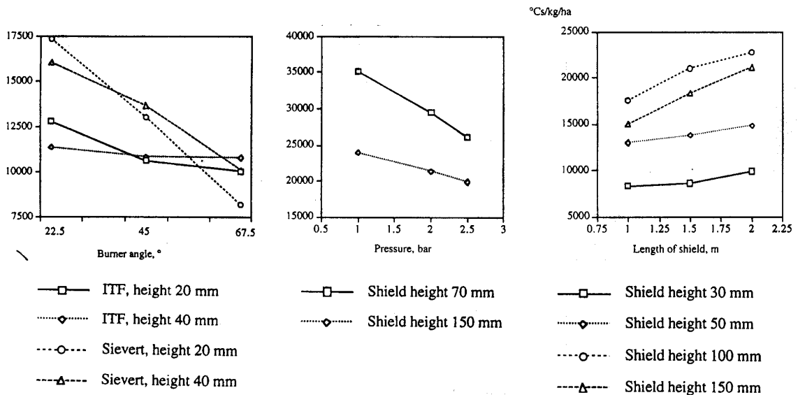
Figure 4. Relative utilization factor ( \frac{??T \times t}{G} = \text{Cs/kg gas/ha} ) (Storeheier 1991) Left . Sievert and ITF burners, unshielded and with different burner heights and mounting angles relative to soil surface. Middle . Mean results for the two burner types at different shield heights and gas pressures. Right . Mean results for different shield heights and shield lengths. (Storeheier 1993)
